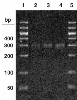
Fig. 2. Formation of the full-library. Four 30-mer oligonucleotide "splints" were obtained (IDT) with sequences: \bar{X}^T_{11}, \bar{X}^T_{10}, \bar{X}^T_{11}, \bar{X}^F_{10}, \bar{X}^F_{11}, \bar{X}^T_{10}, \bar{X}^F_{11}, \bar{X}^F_{10} . Ten pmol of each half-library was mixed with 2 pmol of each of the four splints, in a final volume of 25 \mu l in 1 \times T4 DNA ligase buffer (Promega, Madison, WI) (note: no ligase was added) and incubated at room temperature for 2 hours. One-half microliter of the mixture was PCR-amplified with primer set: \langle X^T_1, X^F_1, \text{Acrydite-modified } \bar{X}^T_{20}, \text{Acrydite-modified } \bar{X}^F_{20} \rangle , under standard conditions for 35 cycles. Then, 1- \mu l aliquots were PCR-amplified from the product above, using the above primer set, under standard conditions for 35 cycles. The products were run on a 1% agarose gel, the 300-bp band extracted with Ultrafree-DA DNA extraction kit (Millipore, Bedford, MA), then pooled to create a stock solution with a final volume of \sim 500 \mu l. Another round of PCR amplification was performed using the above primer set under standard conditions for 15 cycles with 2.5- \mu l aliquots of stock solution as template. The resulting DNA was ethanol-precipitated and rehydrated in 75 \mu l of water. Shown here are 1 \mu l (lane 2), 2 \mu l (lane 3), and 3 \mu l (lane 4) aliquots of the full library run on a 4% agarose gel. Lanes 1 and 5 are molecular weight markers.
