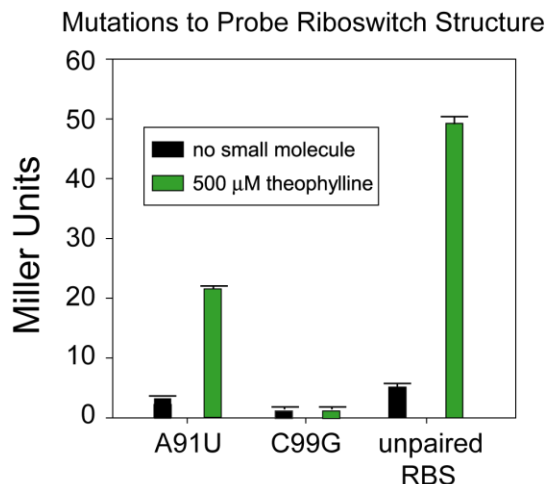
Figure 2.7: Structure Probing Mutations. Mutations were introduced into the riboswitch with an 8 base pair linker between the aptamer and RBS, based on the mFold structure. A91U was predicted to slightly unpair the RBS; C99G was predicted to pair the RBS; and the “unpaired RBS” construct was made by mutating the codons which were predicted to pair with the RBS. A91U functioned in a theophylline dependent manner, as expected. C99U was not theophylline responsive, as expected. The unpaired RBS constructed was theophylline responsive, which was not expected.
