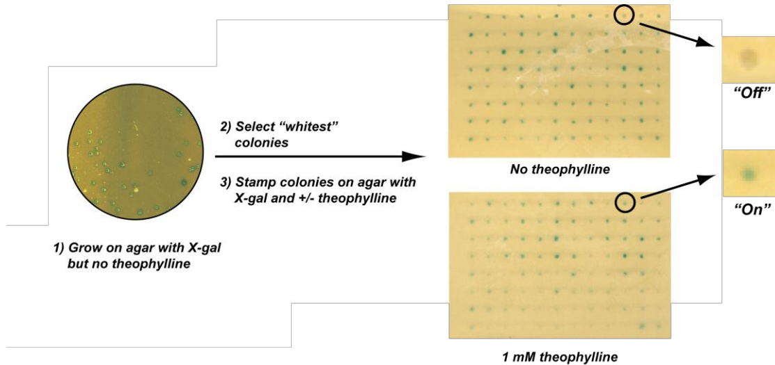
Figure 3.4: Diagram of the High-Throughput “Stamping” Assay. E. coli cells harboring potential riboswitches (cloned upstream of IS10-lacZ ) are plated onto selective agar supplemented with X-gal. A colony-picking robot is used to pick the whitest colonies (low levels of \beta -galactosidase activity). These colonies are stamped on agar supplemented with X-gal and either no small molecule or theophylline (1 mM). After growth, colonies that are blue only in the presence of theophylline are assayed further.
