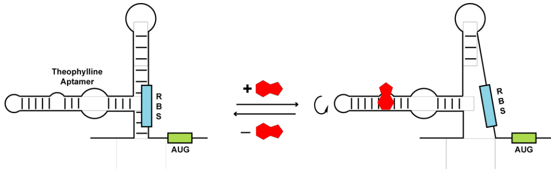
Figure 1.9: Mechanism of a Theophylline-Activated Riboswitch. Workers from the Sues group designed a theophylline-activated riboswitch in B. subtilis based on helix slippage. In the absence of theophylline, the RBS is paired, and gene expression is inhibited. However, when theophylline is present (red), it binds to the aptamer and causes a slippage of the paired RBS by one base, resulting in an unpaired RBS and translation begins.
