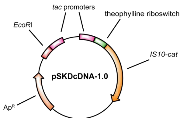
Figure 5.3: Theophylline-selectable cDNA Cloning Vector. When introduced into E. coli , the vector provides resistance to chloramphenicol, only in the presence of theophylline. The vector also contains a single EcoRI site for cloning of PCR-amplified cDNA, under the control of a constitutive tac promoter. In pSKDcDNA-1.0, the theophylline riboswitch has 8 base pairs between the ribosome-binding site and the aptamer, as reported. 3
