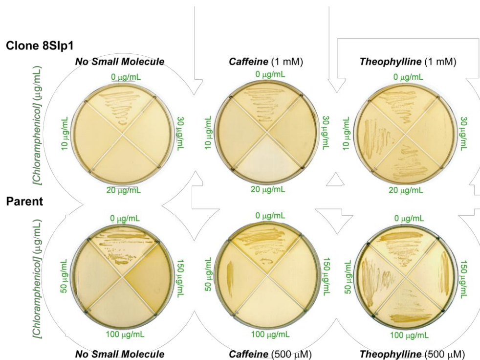
Figure 3.7: Resistance Assays with the Parent and 8SIp1 Riboswitches. E. coli cells harboring either the parent or 8SIp1 synthetic riboswitches, cloned upstream of the chloramphenicol resistance gene ( cat ), were grown on agar supplemented with varying chloramphenicol concentrations and small molecules. Riboswitch 8SIp1 requires lower concentrations of chloramphenicol than the parent riboswitch. Clone 8SIp1 also displays no background growth in the presence of caffeine with any concentration of chloramphenicol, unlike the parent.
