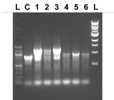
Figure 5.6: PCR Reactions of Colonies that Survived Selection on Caffeine. The agarose gel (1%) contains a 100 bp ladder (left lane), 1 kb ladder (right lane) and a vector only control (C). Colonies 1-3 contain cDNA inserts, while colonies 4-6 do not. The cDNA inserts were found to be non-coding.
