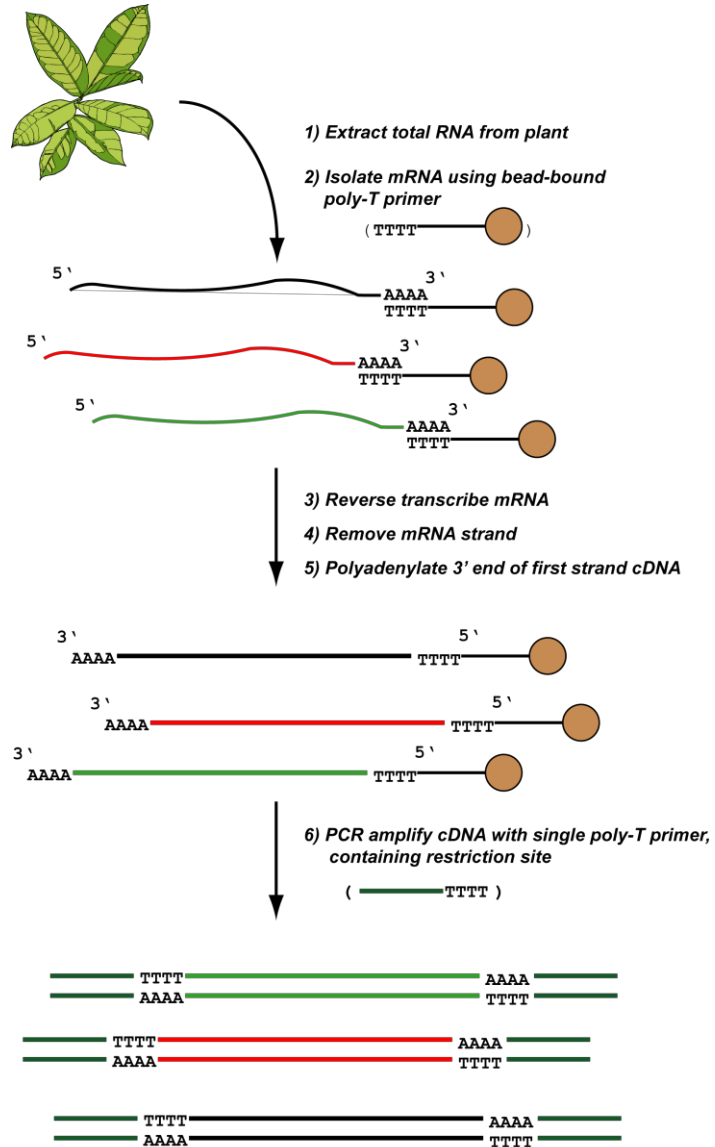
Figure 5.4: cDNA Synthesis Scheme. Total RNA is extracted from C. arabica and is converted into a double-stranded DNA product with terminal restriction sites.
