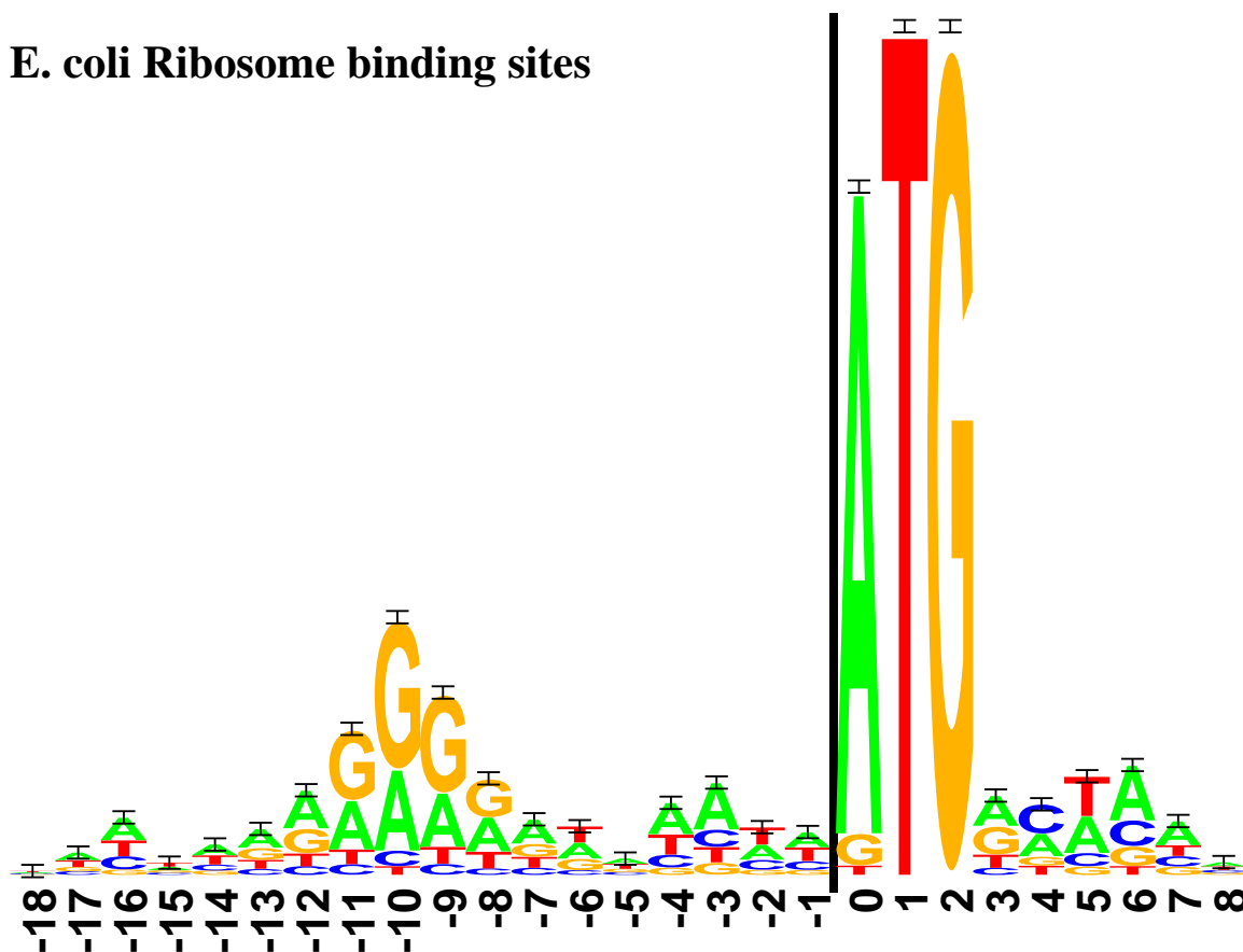
Figure 1: Logo for E. coli ribosome binding sites. Only -18 to +8 of the -20 to +13 site is shown. The first translated codon is just to the right of the 2 bit high vertical bar. 149 natural sites were used to create the logo [9].
