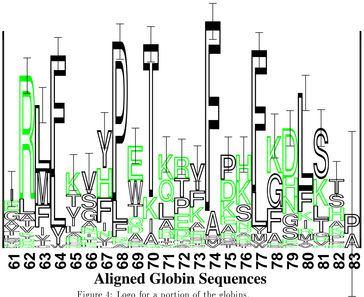
Figure 4: Logo for a portion of the globins.
