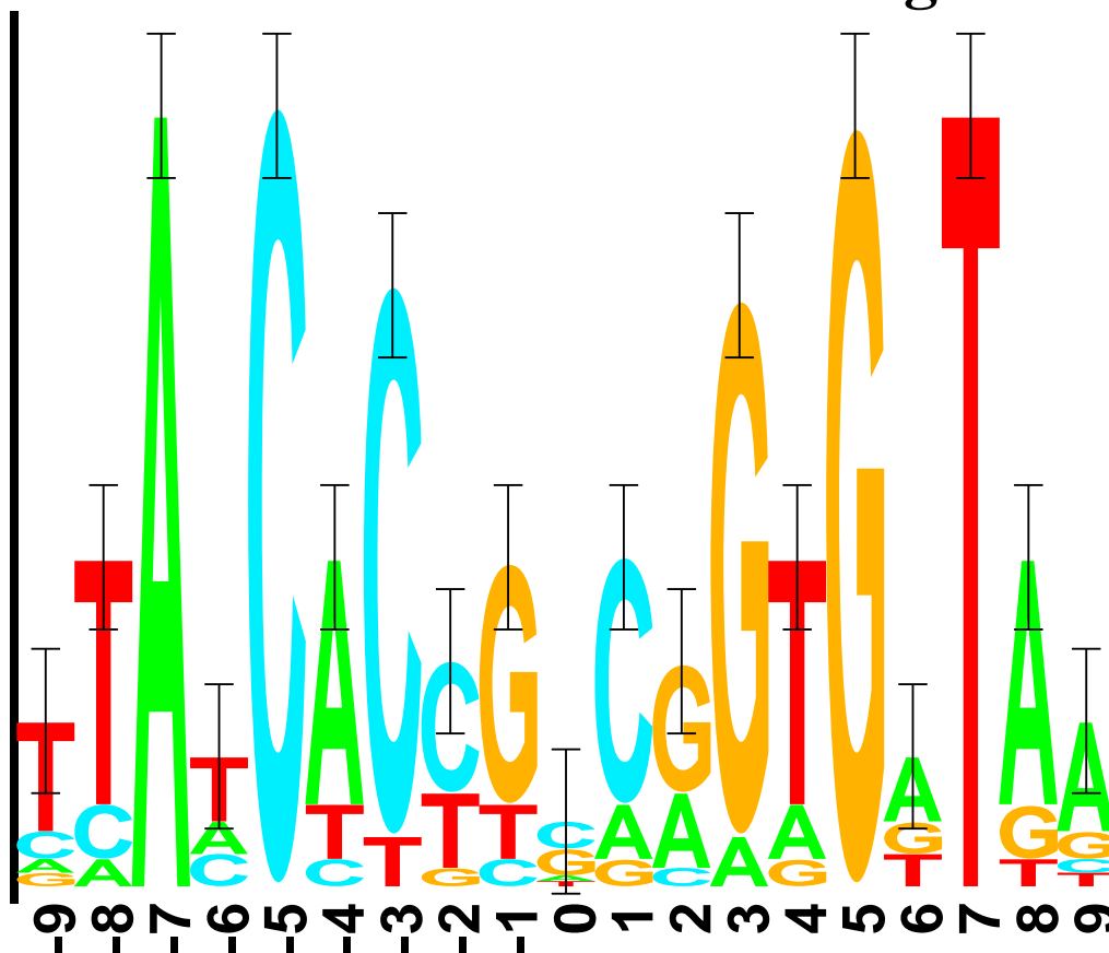
Figure 2: Logo for bacteriophage Lambda cI and cro binding sites. The 6 natural operators and their complementary sequences were used to create the logo [9].
