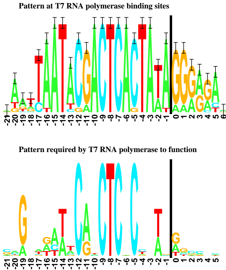
Figure 3: Logo for sequences at T7 RNA polymerase binding sites in the bacteriophage T7 genome (upper logo) and logo for the pattern that is required for T7 RNA polymerase alone to function (lower logo). The first transcribed base is just to the right of the 2 bit high vertical bars. The 17 natural promoter regions were used to generate the upper logo [9]. 53 promoter variants were used to generate the lower logo [12].
